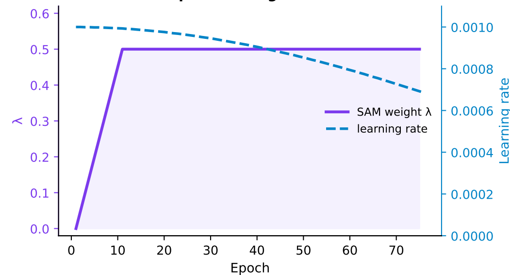
B · \lambda ramp & learning-rate schedule
