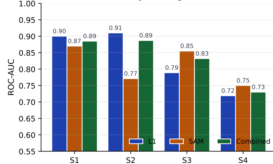
F · AUC by scoring method
