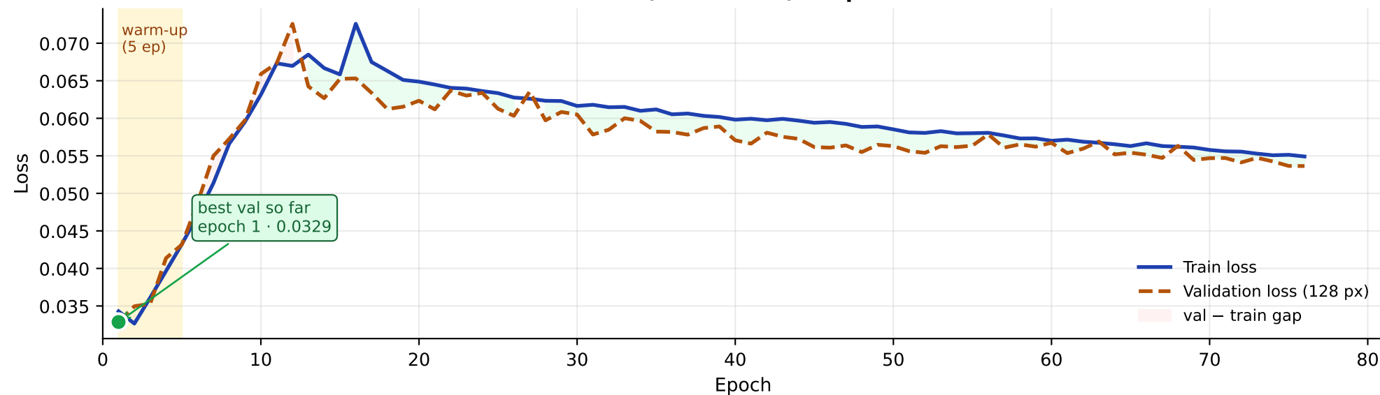
A · Combined loss (L1 + \lambda ·SAM) · epochs 1-76 of 200
